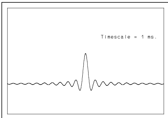
Figure 11: Impulse response of Brick-Wall filter.
