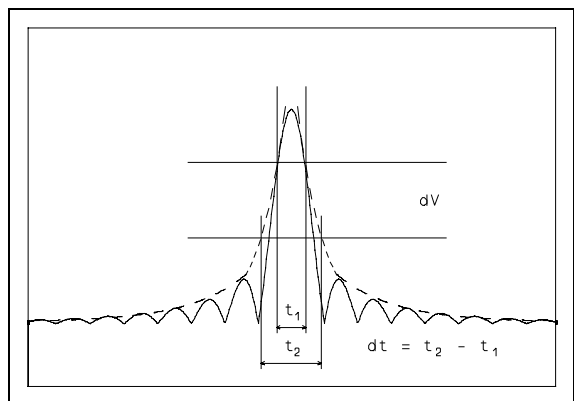
Figure 6: Temporal decay of digital filter.
