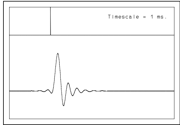
Figure 14: Impulse response of filters of fig. 12 and 13 in series, simulating the effect of a digital audio chain (recording + playback).
