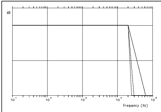
Figure 7: Frequency responses of phase linear audio systems with roll-off rates of order 2, 6 and 10.
