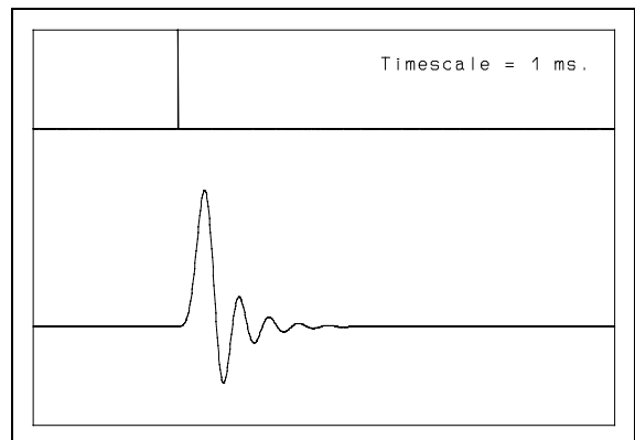
Figure 12: Impulse response of 80 dB/oct. elliptical filter at 20 kHz.
