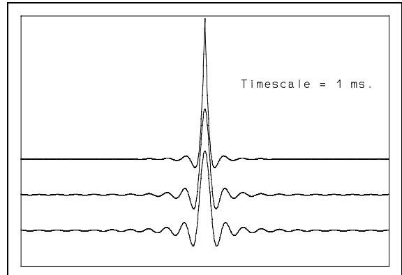
Figure 8: Impulse responses of audio systems with 20 kHz bandwidth but with roll-off orders of 2, 6 and 10.
