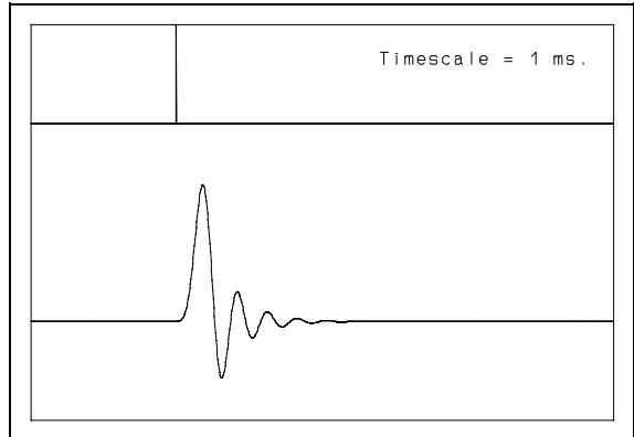
Figure 4: Impulse response of band-limited audio system.
