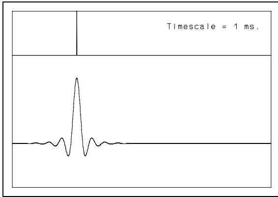
Figure 13: Impulse response of filter of fig. 12, but with the phase shift set to zero for all frequencies.
