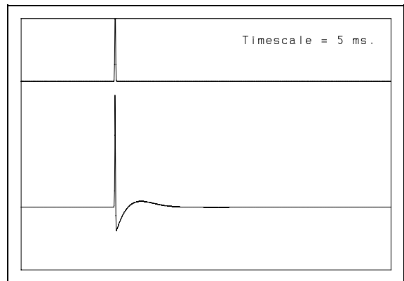
Figure 16: Impulse response of Butterworth cross-over filter of 4 th order at 1 kHz.
